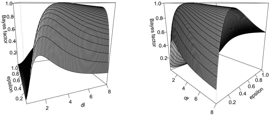
Figure 1: Model assessment for the aspirin and colon cancer data. The Bayes factor as a function of v , the number of degrees of freedom in (3.3a), and \epsilon , the common value of c_1 and c_2 in the gamma prior in (3.3b), is shown from two different angles. Here the baseline value of the hyperparameter corresponds to v = 4 and \epsilon = .125 .
